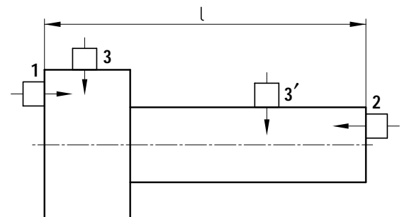
Figure B-4: Scanning positions for rough-turned stepped bolts and trunnions (examples)
