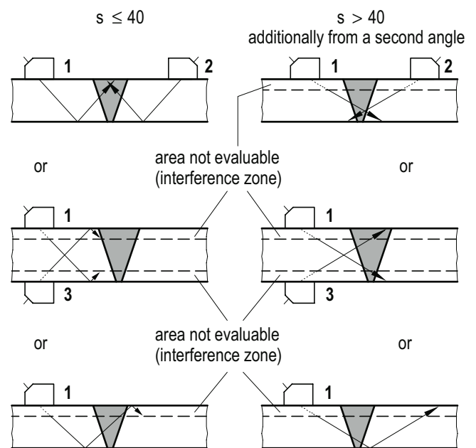
Figure B-5: Scanning positions for butt welds
