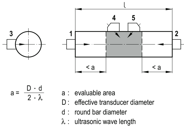
Figure B-2: Scanning positions for round bars
