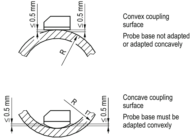
Figure B-1: Adaptation of probe base to curved surfaces
