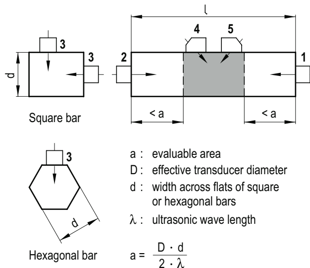
Figure B-3: Scanning positions for rectangular or polygonal bars
