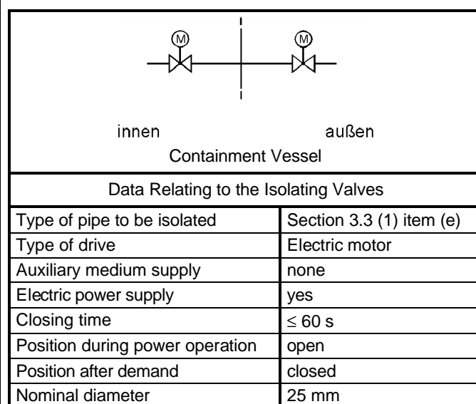
Fig. A-8: Example of an arrangement of isolating valves for the off-gas system of pressurized water reactors
