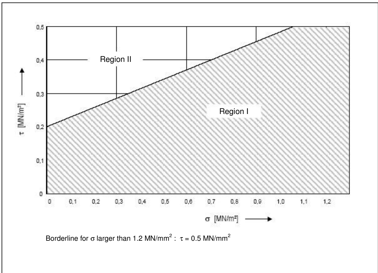
Figure 4-1: Shear stress, \tau , as specified under Section 4.1.2 and the corresponding normal stress, \sigma , in case of a dynamic surface loading condition
